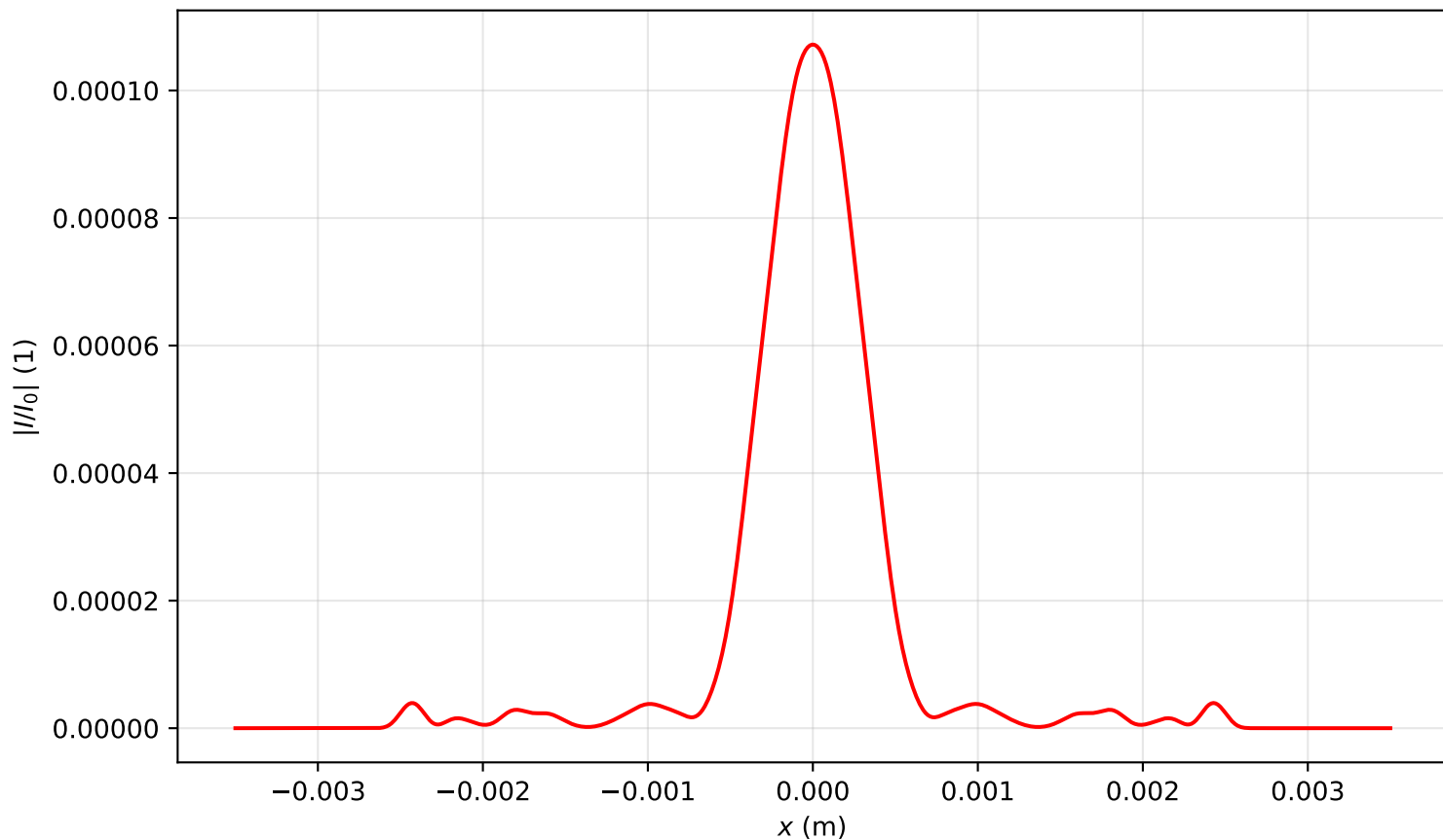
Intensity profile I(x, y = 0, z = 1.911)/I_0 , P_{in}=9.0P_{cr} , artificial time
